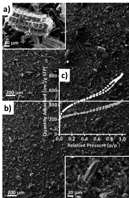
Fig. 1 Representative SEM images of C_{\text{W}} (a) and C_{\text{Chemical}} (b). (c) N_2 physisorption isotherms collected at 77 K for C_{\text{W}} (grey) and C_{\text{Chemical}} (white).
